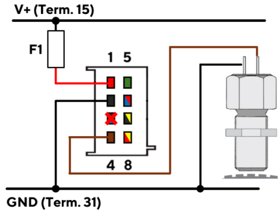
Pull-Up Input
